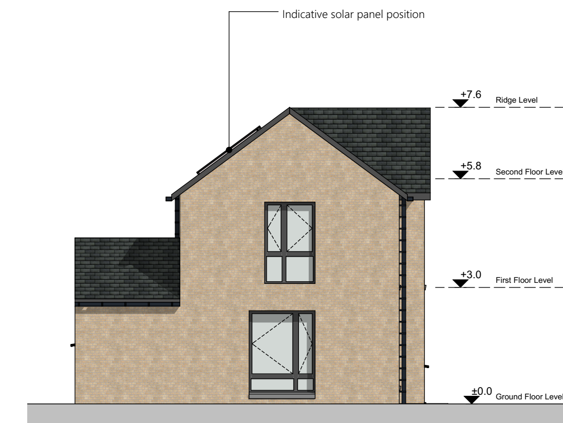
Side Elevation 1 SCALE 1:100
