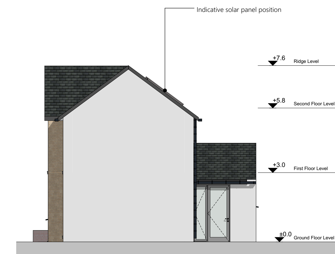
Side Elevation 2 SCALE 1:100
