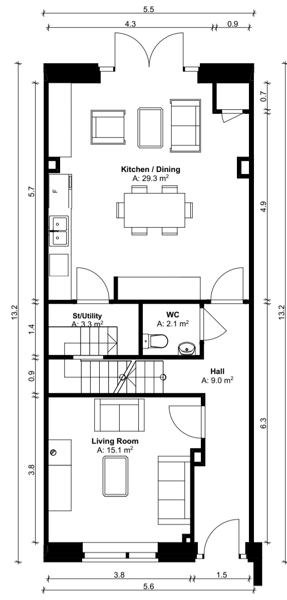
HOUSE TYPE A - 64.3M 2
